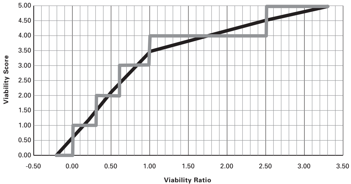
Figure 1. Viability Scores
